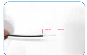
2.8 The fiber length specification
